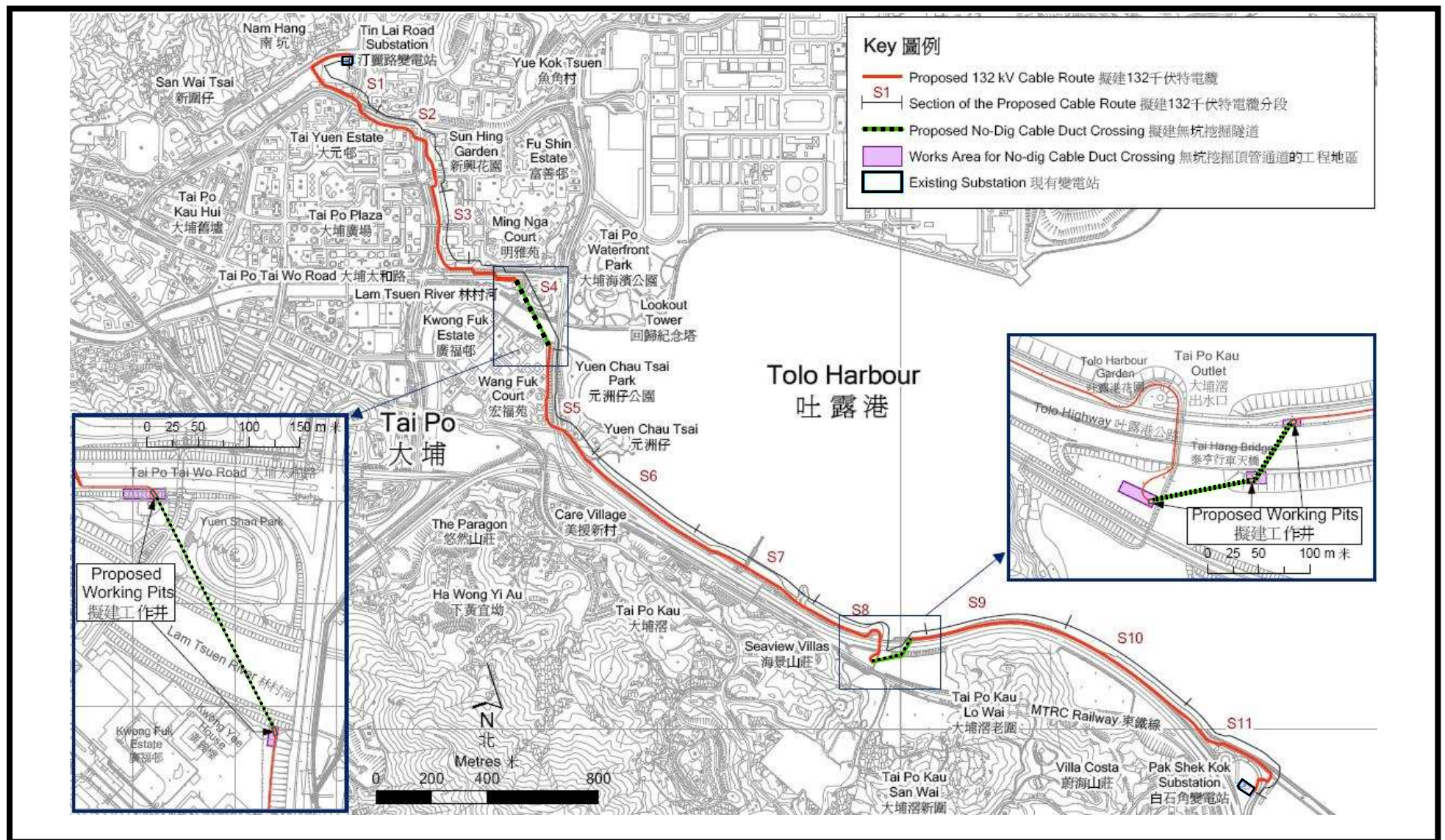
Figure 1 Installation of the Proposed 132kV Cable Circuit Connecting with Ting Lai Road Substation and Pak Shek Kok Substation (連接汀麗路變電站至白石角變電站的 132 千伏特電纜鋪設工程)
